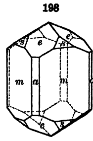
Rutile, First and Second Order Prisms and Pyramids
